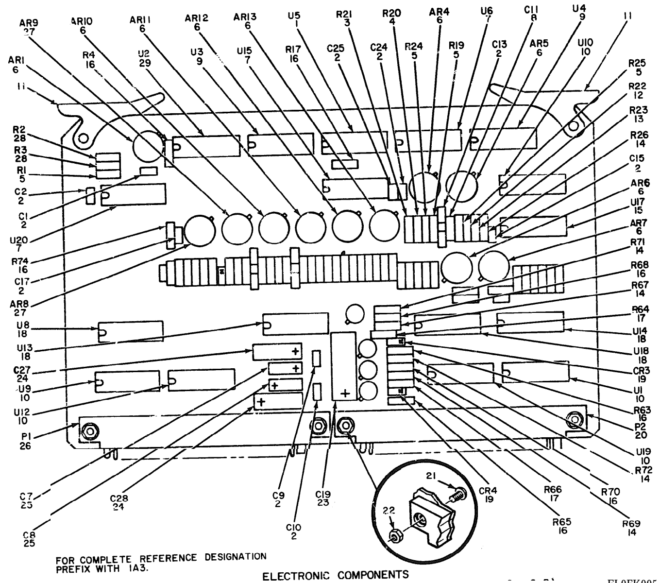
13 Figure 5. Circuit Card Assembly, AGC Processor (1A3) (Sheet 1 of 2).
