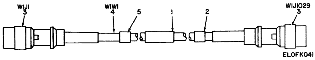
Figure 29. Cable Assembly, RF Antenna W-1.
