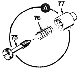
PANEL FASTENING ASSEMBLY
