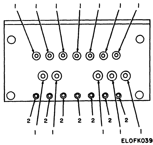
Figure 27. Adapter, Connector Assembly (2) Terminal Board.
