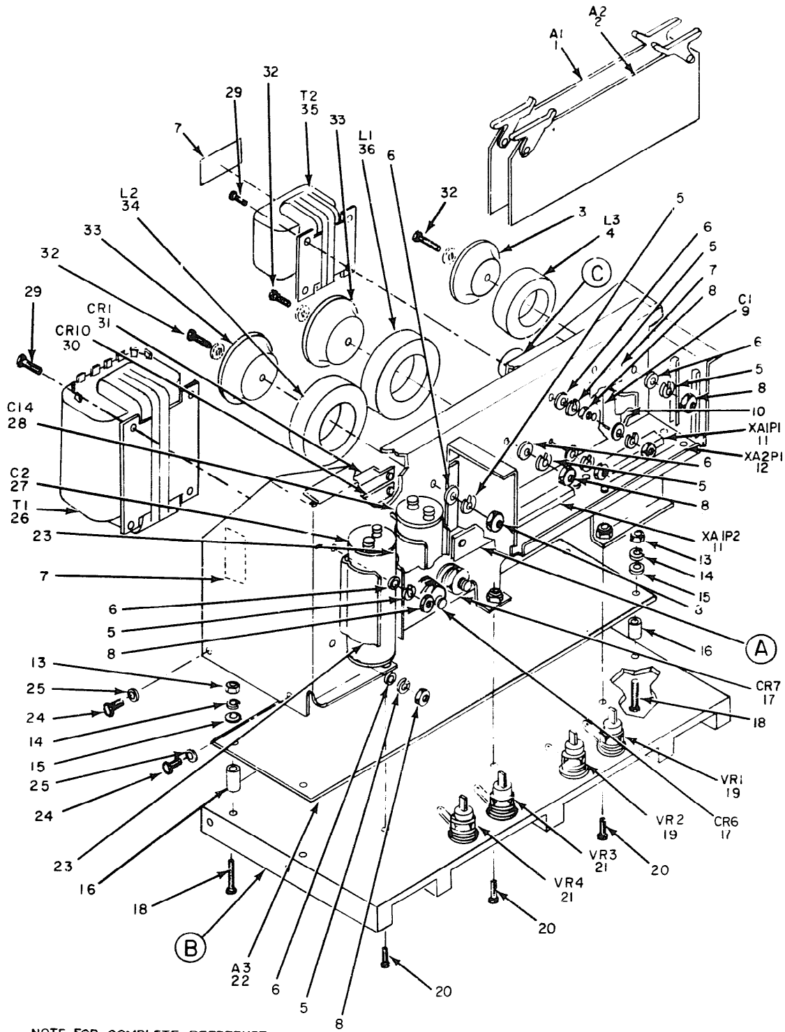
Figure 21. Power Supply (1PS1) (Sheet 1 of 3).
