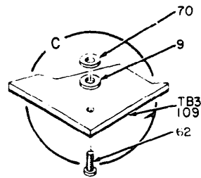
TERMINAL BOARD
