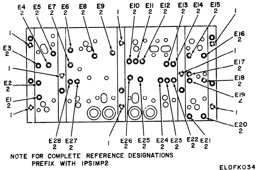
Figure 22. Power Supply (1PS1) Heat Sink, Rear View.
