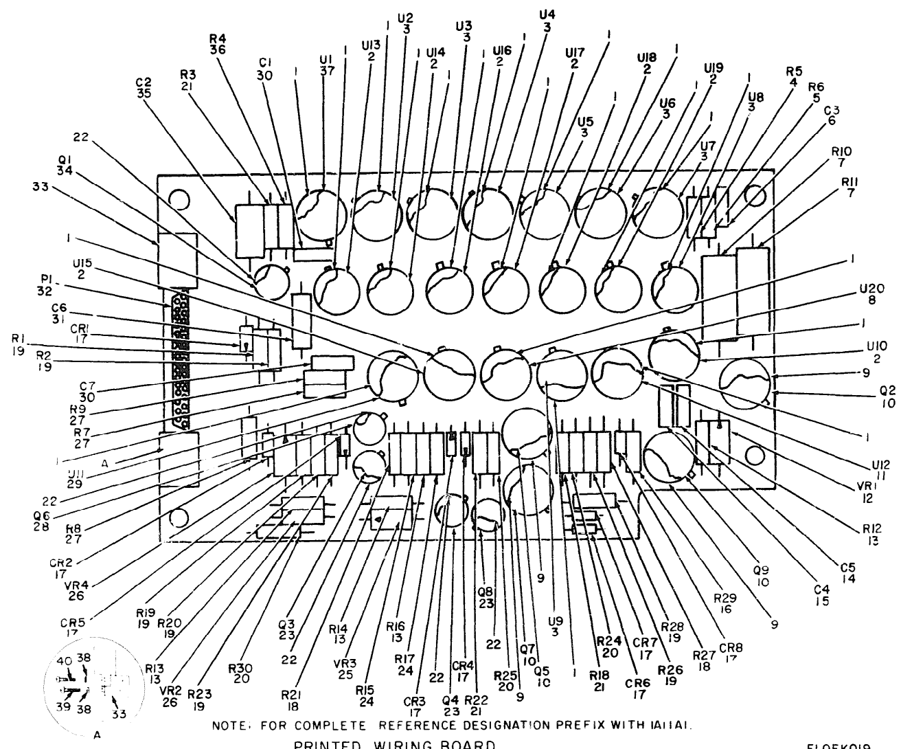
Figure 14. Serial Data Generator (1A11A1).
