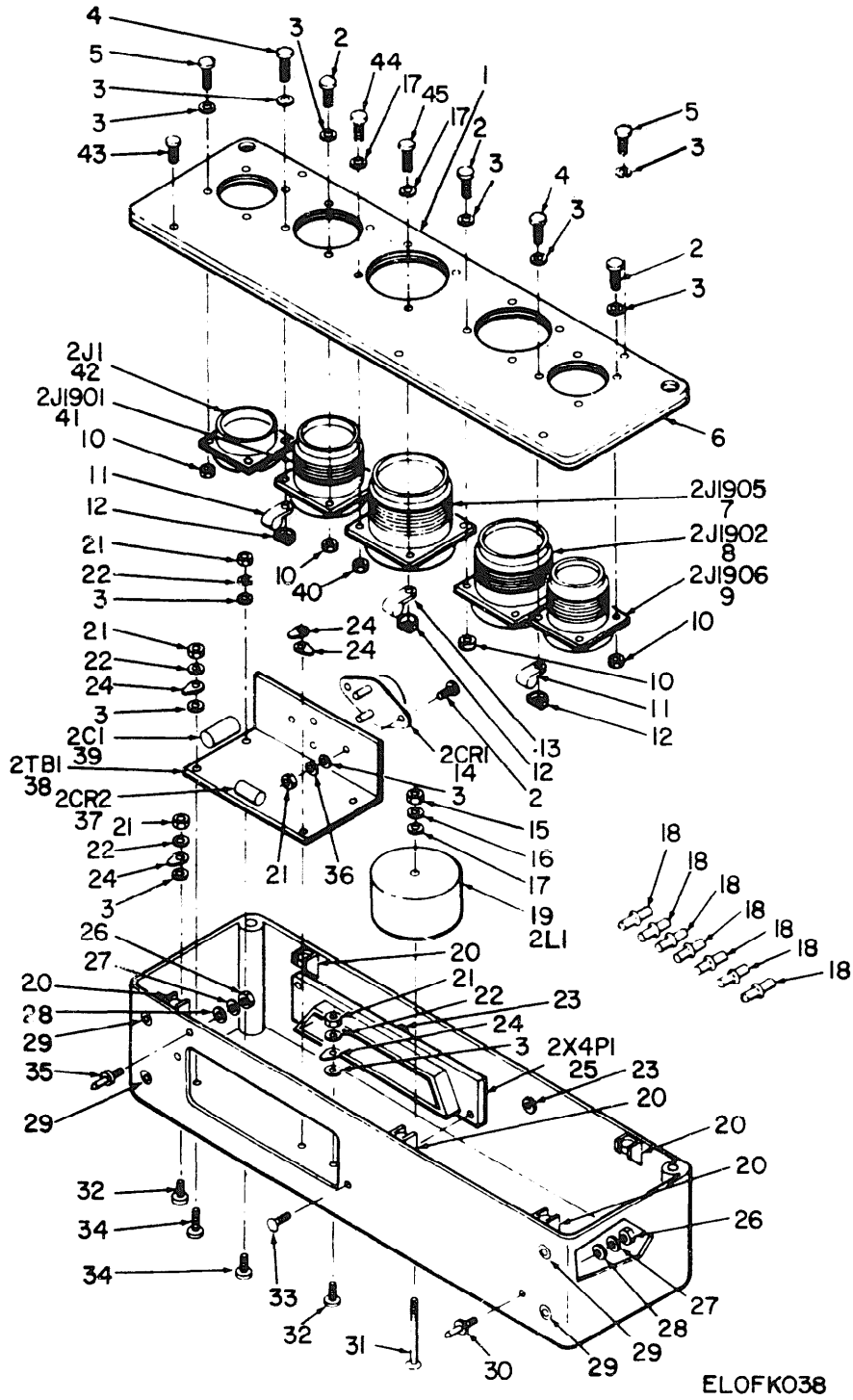
Figure 26. Adapter, Connector Assembly (2).
