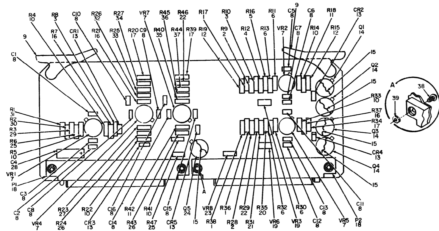
Figure 23. Circuit Card Assembly, Regulator and Delay (1PS1A1).
