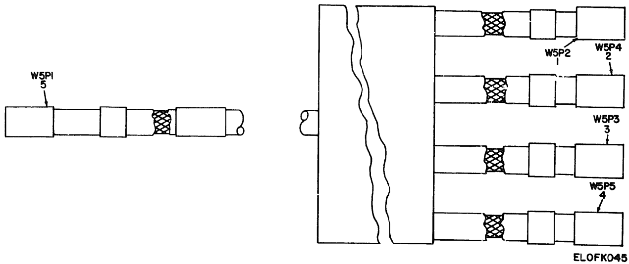
Figure 33. Cable Assembly, Branched, Electrical (Tacan Power) W-5.
