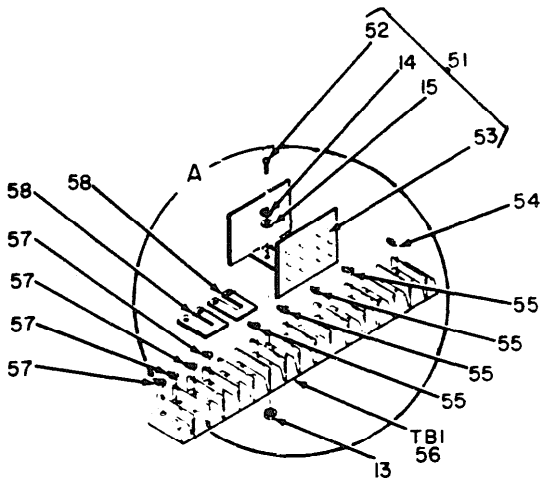
Figure 21. Power Supply (1PS1) (Sheet 2 of 3).
