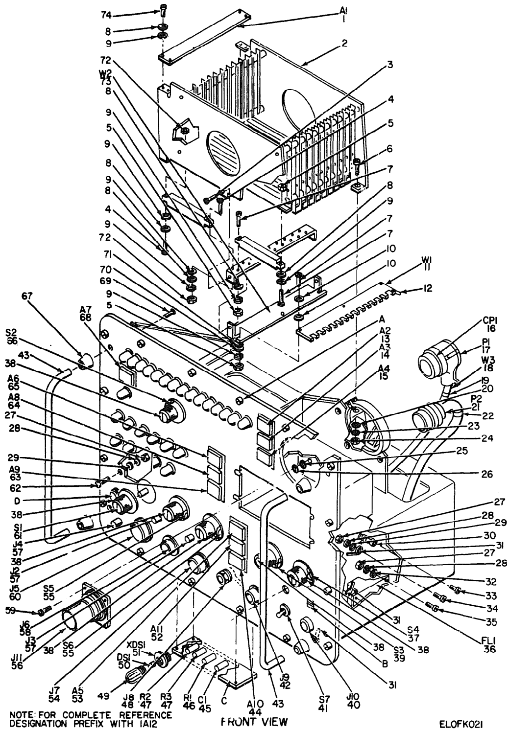
Figure 16. Chassis Assembly, Electrical Equipment (1A12) (Sheet 1 of 4).
